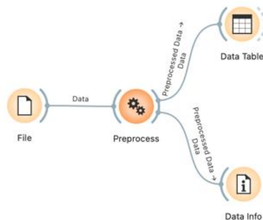
Gambar 3. Preprocessing Data
